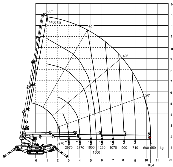
MCX90 + winch load chart
