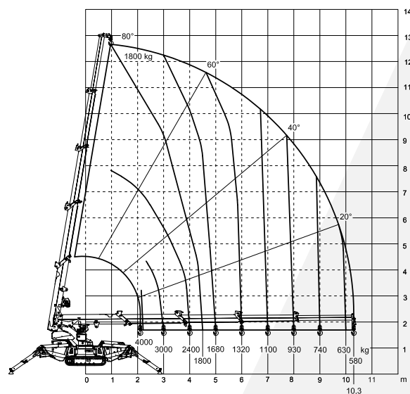
MCX90 + hook load chart
