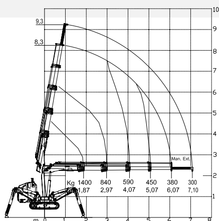
MCR40 narrow stabilization loading chart
