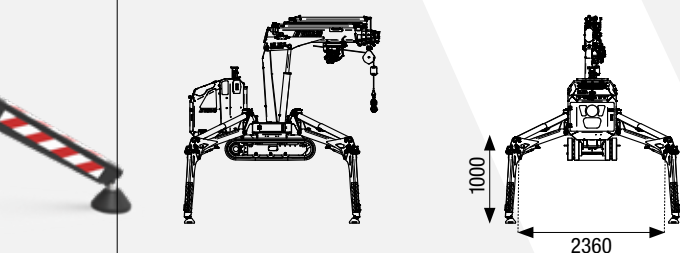
Self-loading dimensions
