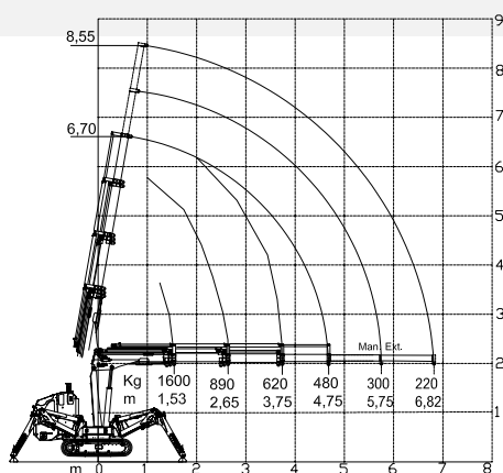
MCR30 Plus narrow stabilization + Winch 800kg load chart
