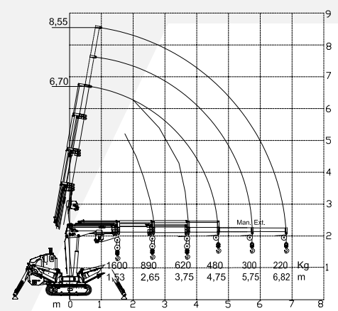
MCR30 Plus narrow stabilization load chart
