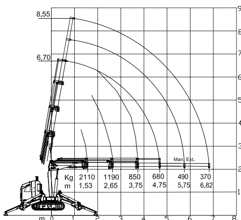
MCR30 Plus load chart
