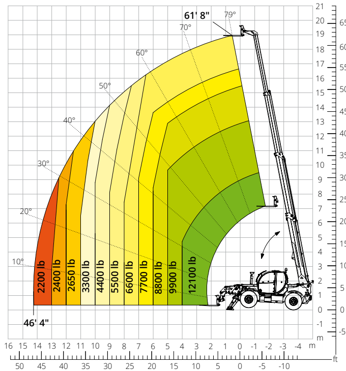
Load chart with WINCH, 13,200 lb ATT-02-004
