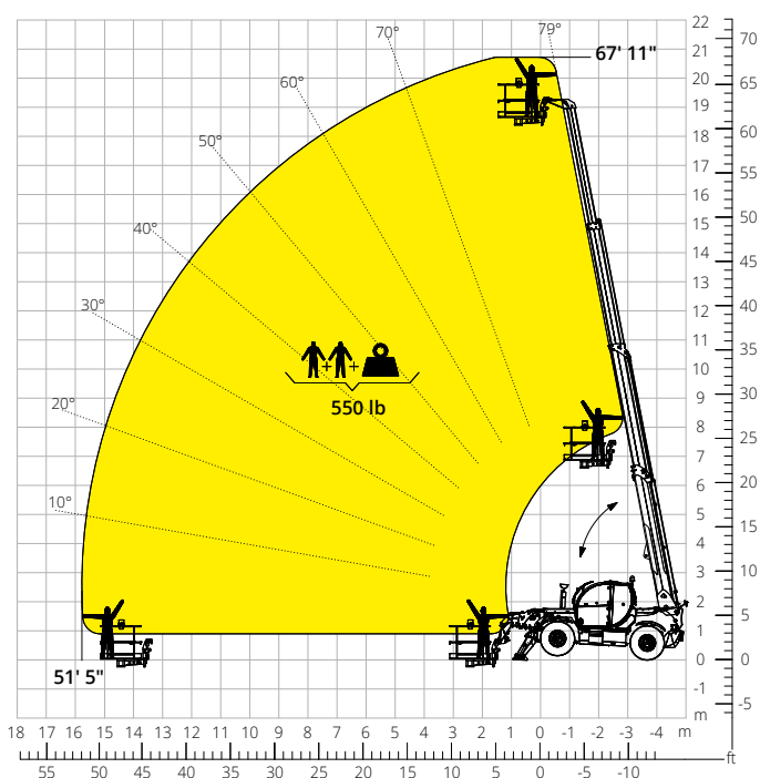
Load chart with FIXED EXTENDABLE PLATFORM, 550 lb ATT-01-003
